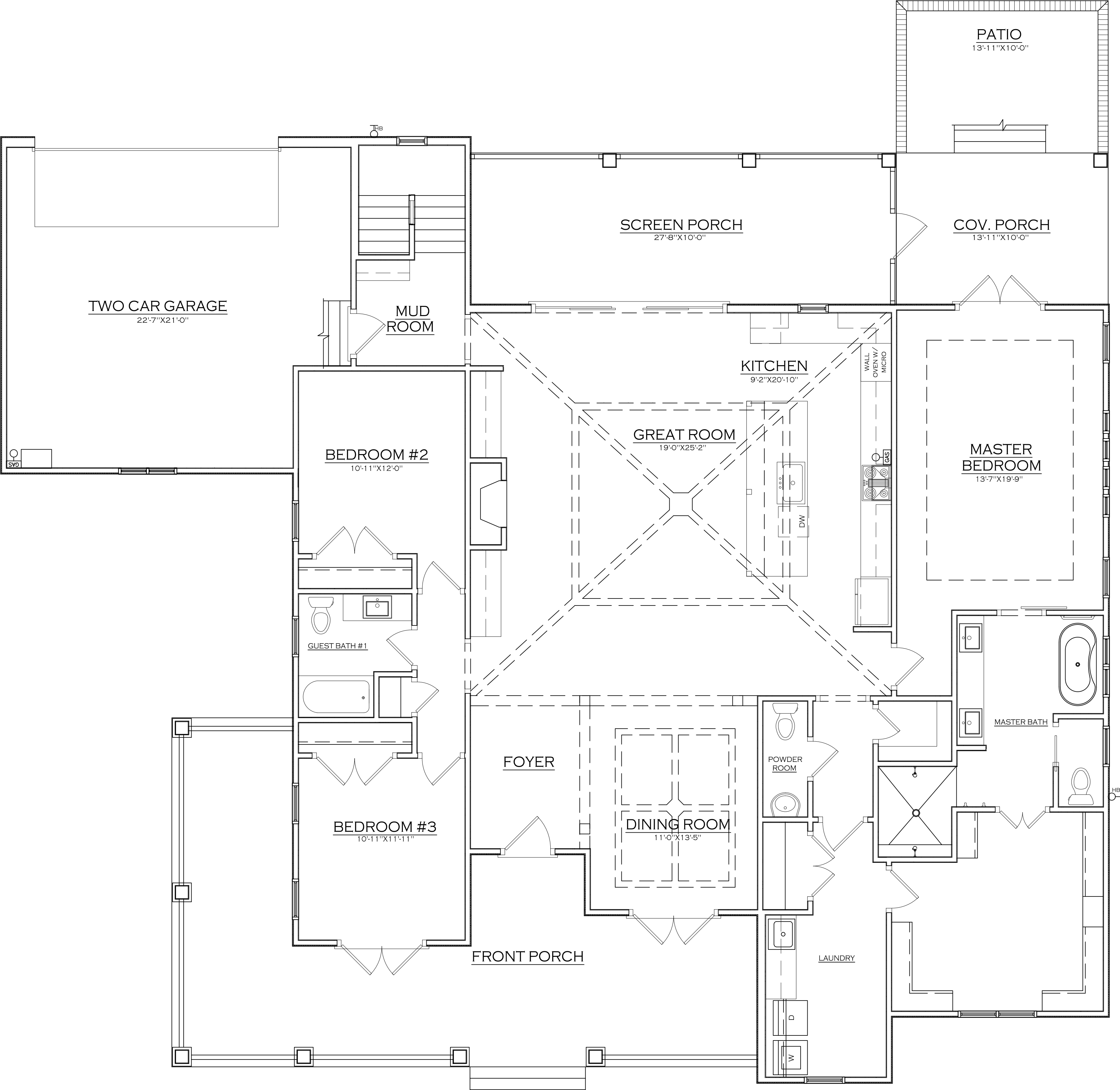
FLOOR PLAN
