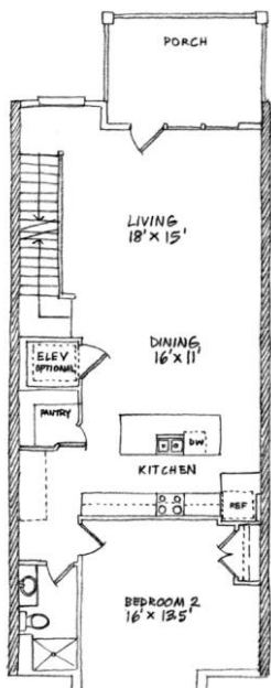
UNIT B FIRST FLOOR PLAN
