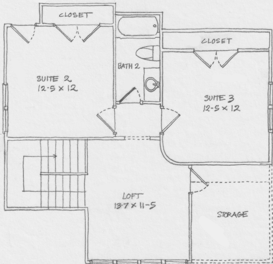
LOT 149 SECOND FLOOR PLAN
