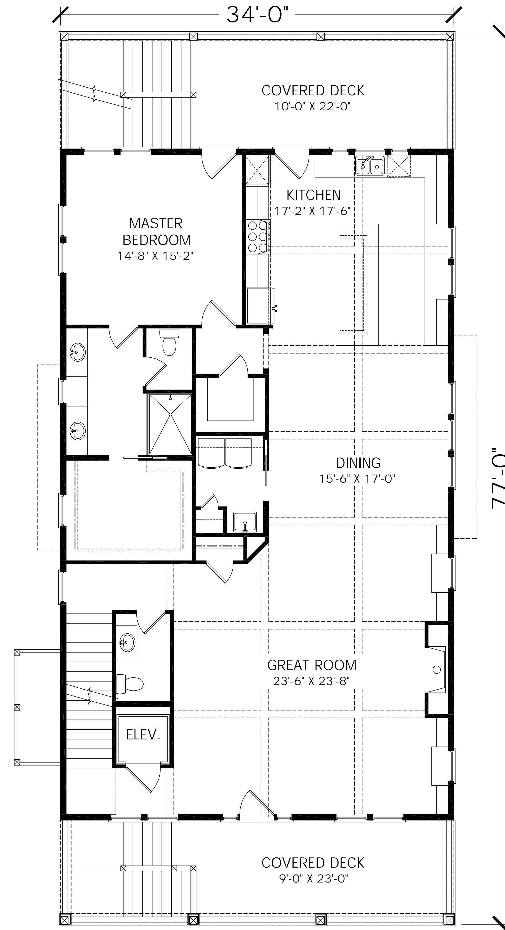
1ST FLOOR PLAN 1,972 SQ.FT.
